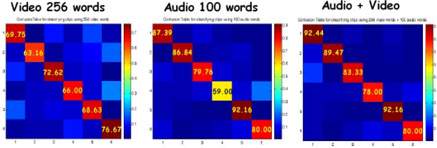
Fig. 2. Confusion Table for 6-class classification using 256 video words(left), 100 audio words(middle), and the combined audio and video words(right). Video words complement audio words to improve the classification performance
