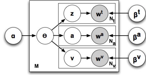
Fig. 1. Graphical model of the proposed Multi-modal Latent Dirichlet Allocation (MM-LDA) model.
